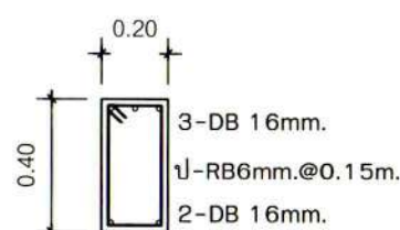
SECTION ③-③
