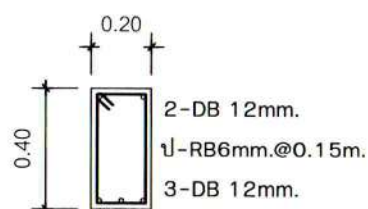
SECTION ②-②
